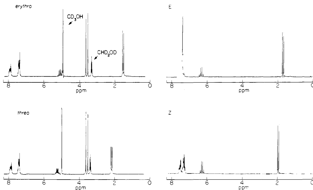
Figure 2. The 100-MHz ^1\text{H} NMR spectra of methyl hydrogen erythro - and threo -1-phenyl-1,2-dibromopropylphosphonic acid in methanol- d_4 and their respective elimination products, ( E )- and ( Z )-1-bromo-1-propenylbenzene in chloroform- d_1 .
